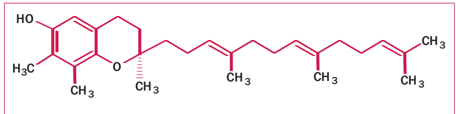
Figure 1: \gamma -Tocotrienol
